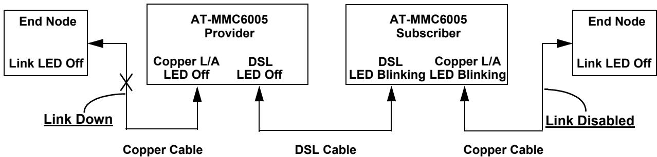
Figure 9. SML with Copper Connection to End Node Down
