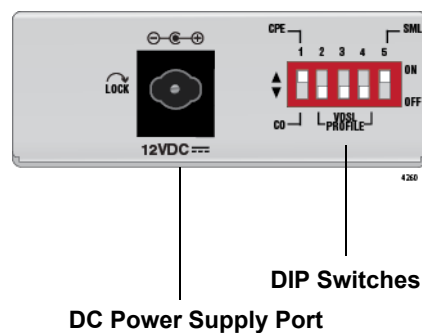
Figure 4. AT-MMC6000 Series Rear Panel
